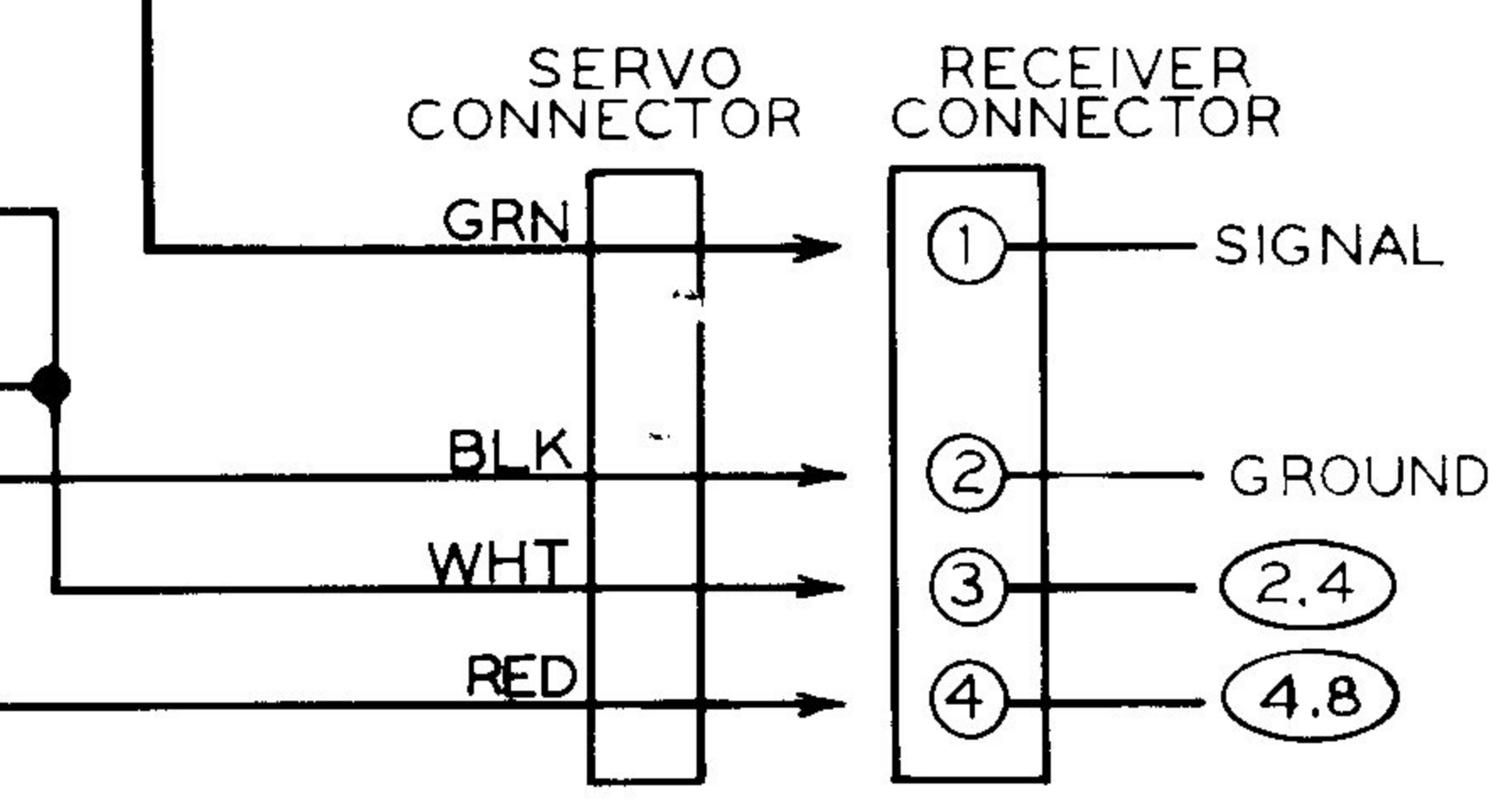
SCHEMATIC OF THE HEATHKIT® SUBMINIATURE DIGITAL PROPORTIONAL SERVO MODEL GDA-19-42
