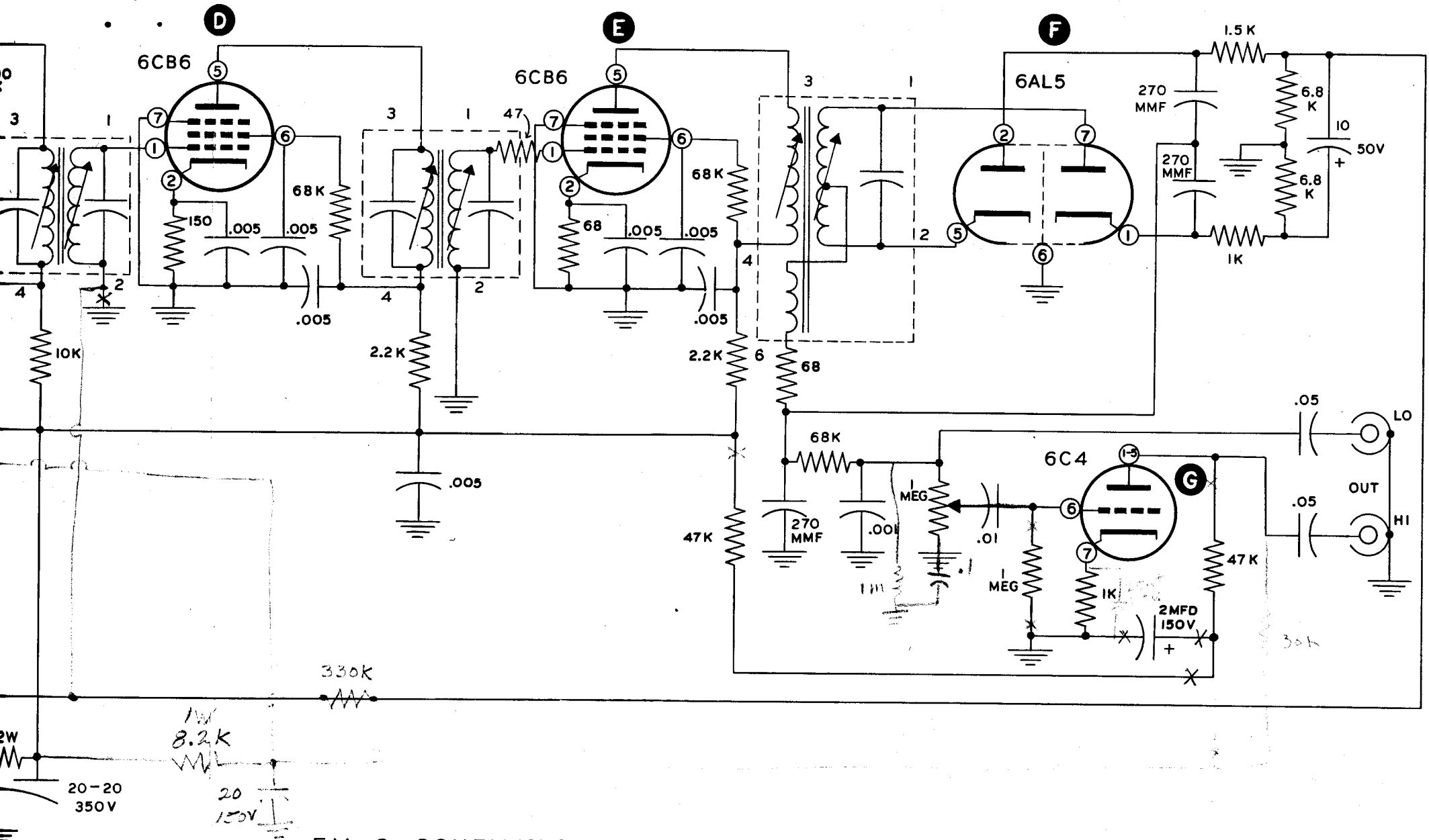
FM-3 SCHEMATIC
