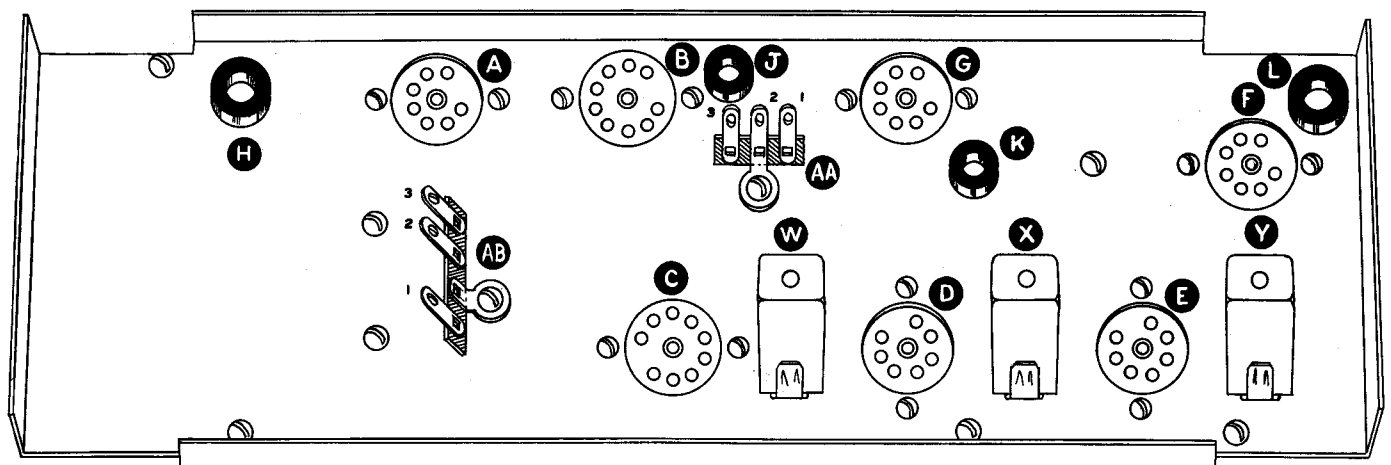
CHASSIS TOP
