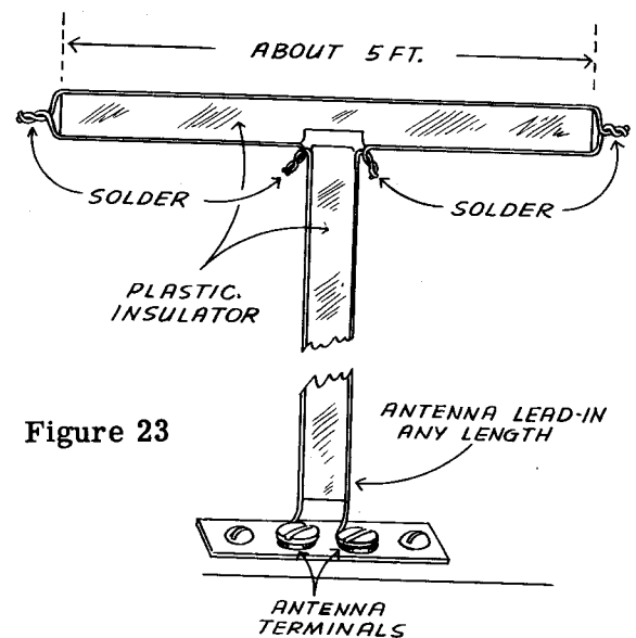
Figure 23 FOLDED DIPOLE ANTENNA MADE FROM 300 OHM TWIN- LEAD TRANSMISSION LINE
