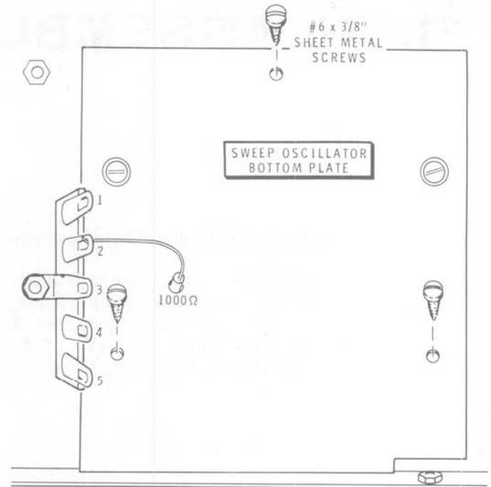
Detail 34B
