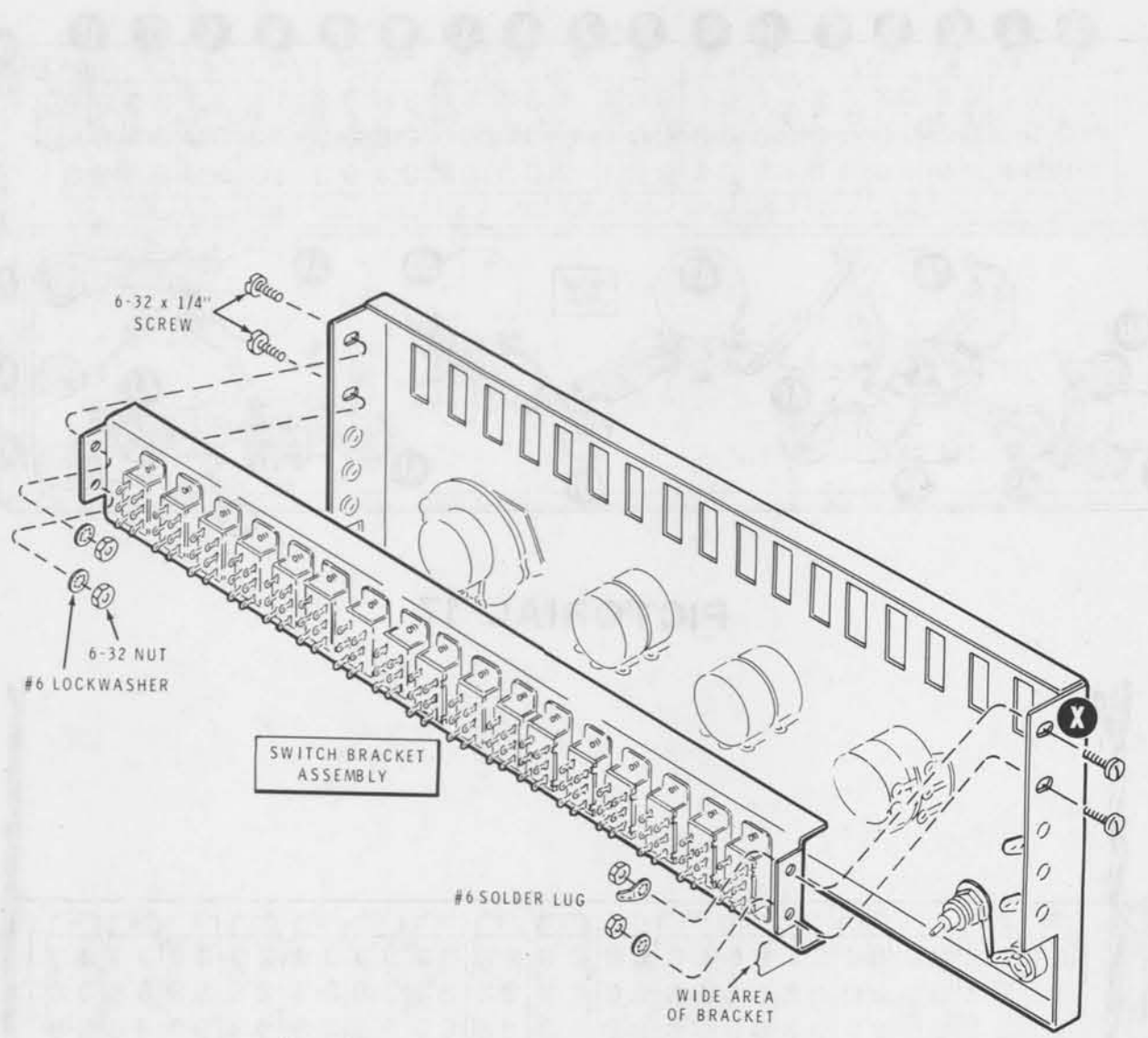
Detail 16J
