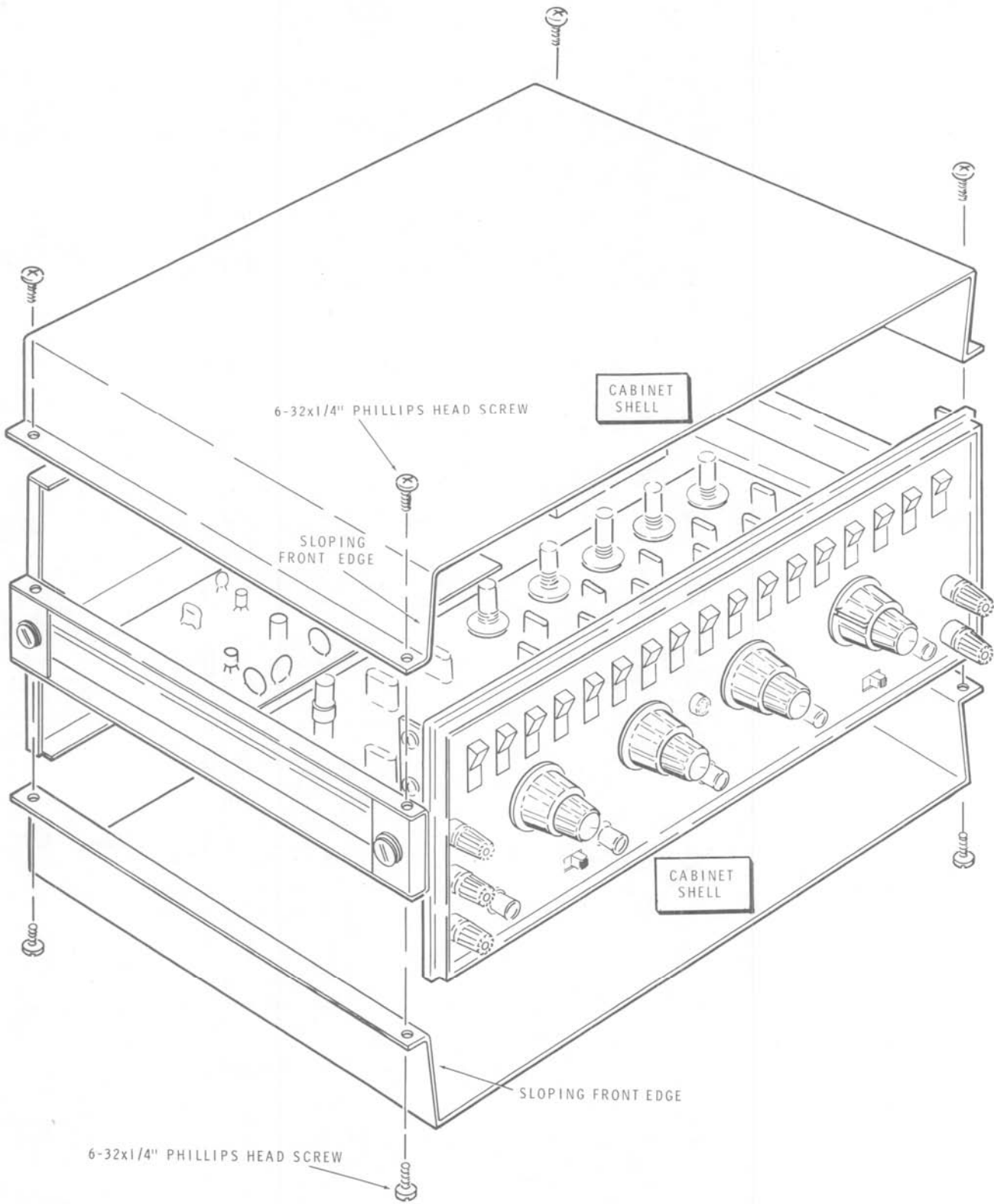
PICTORIAL 34
