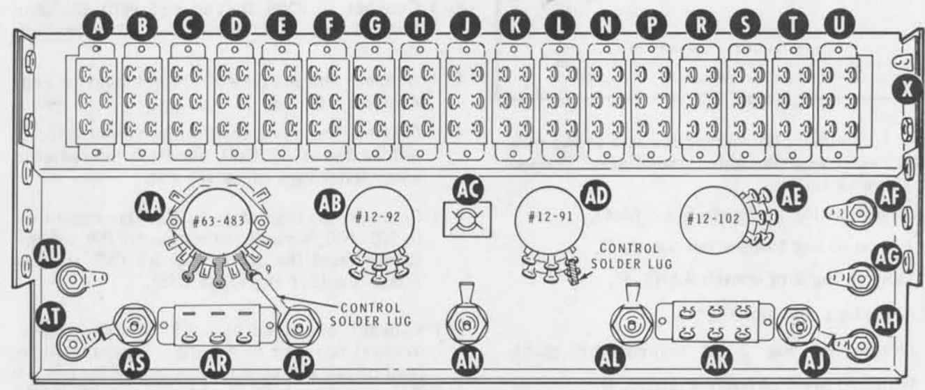
PICTORIAL 16 (Repeat)
