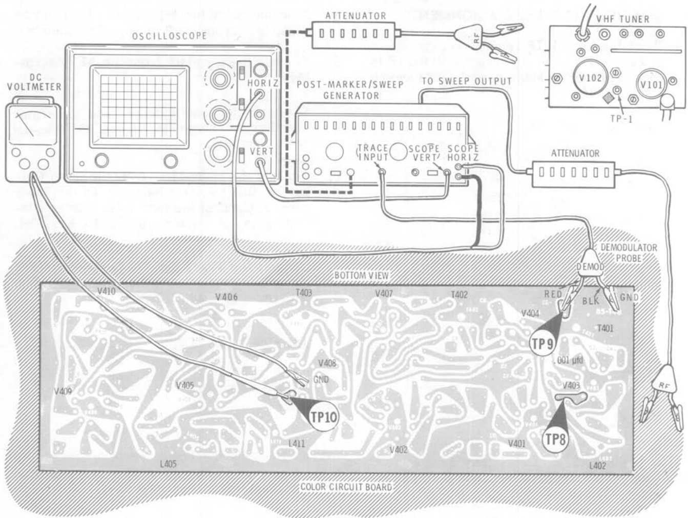
Figure 20 COLOR AND BANDPASS ALIGNMENT
