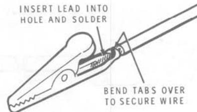
Detail 28D
