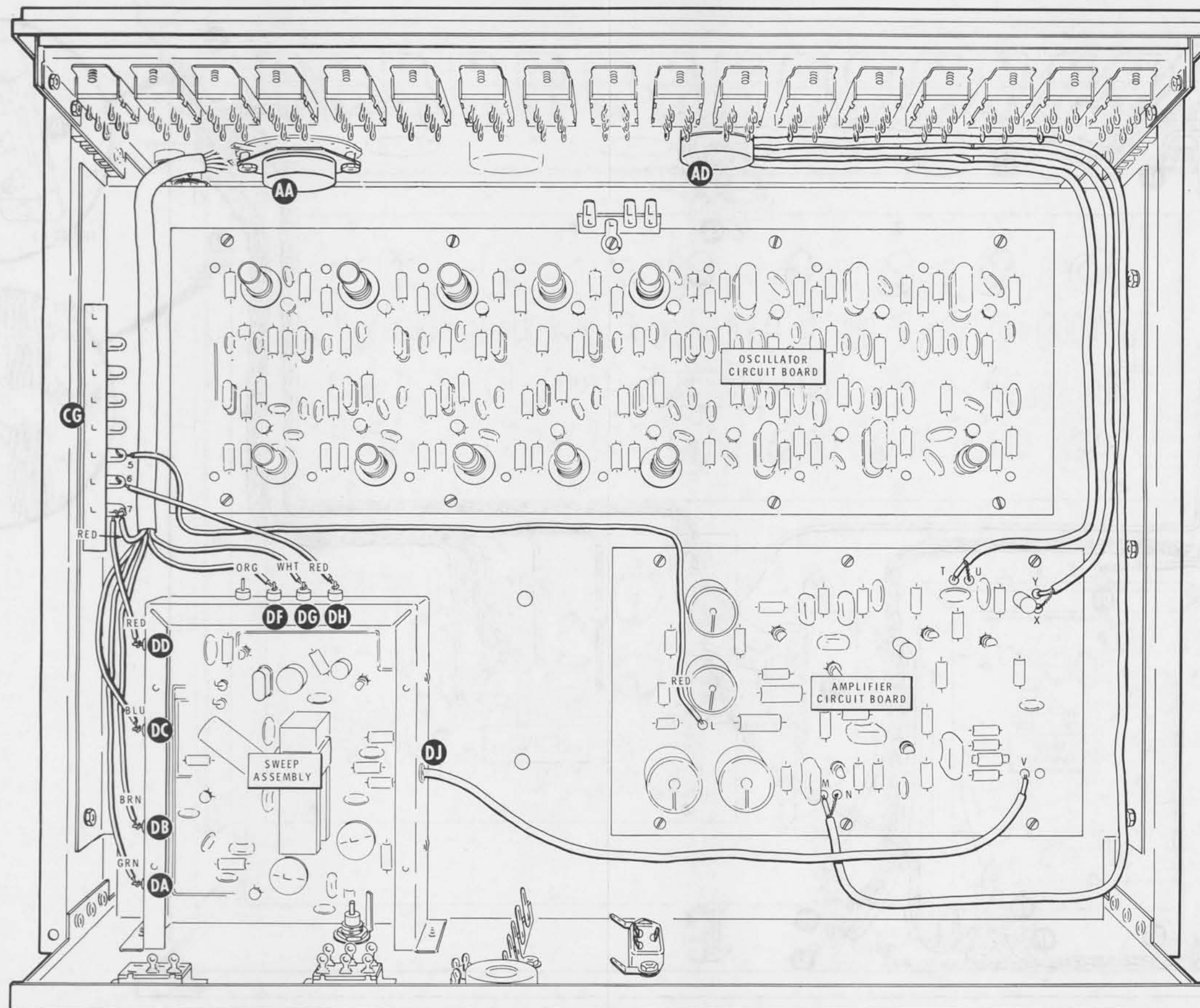
PICTORIAL 23
