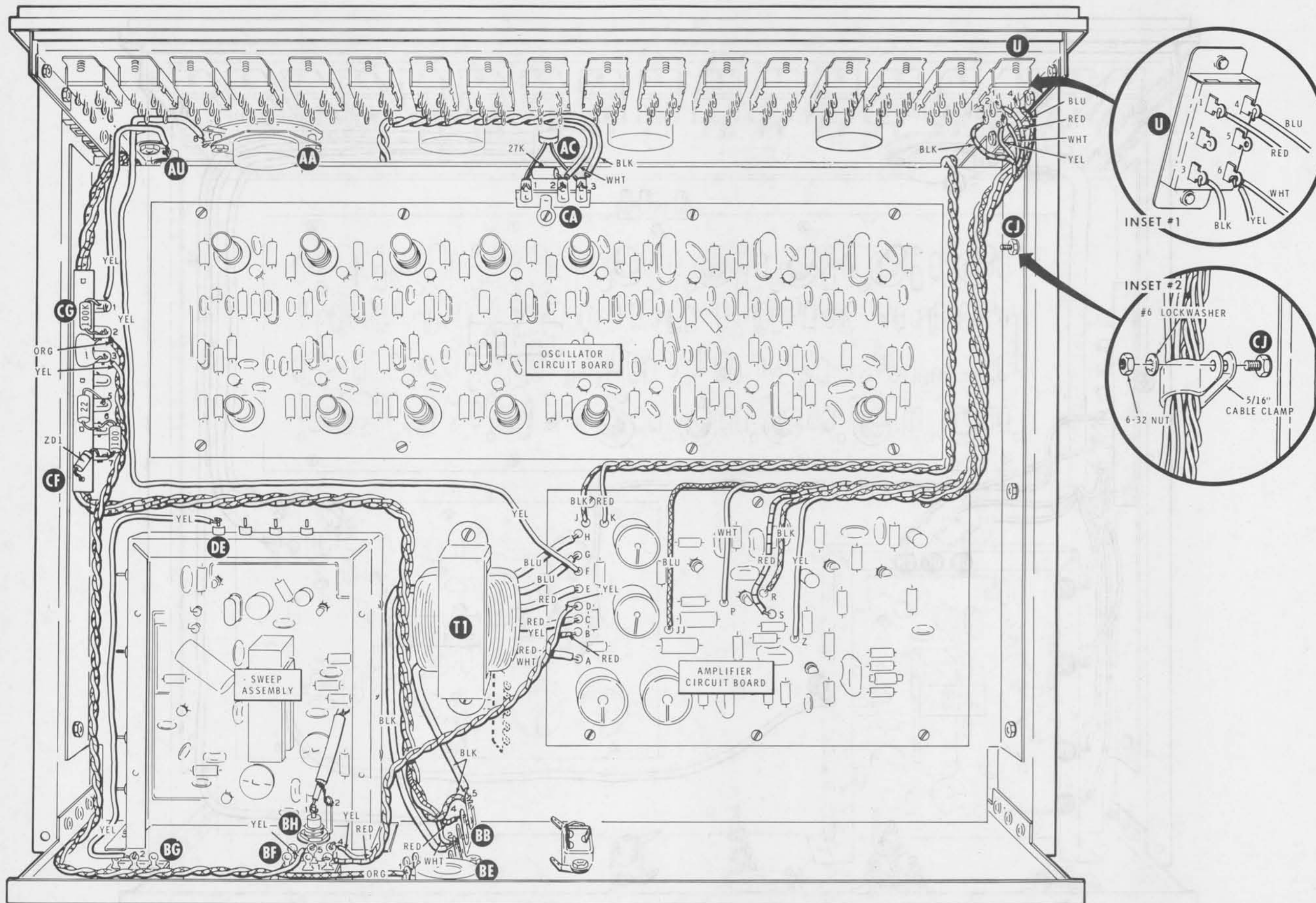
PICTORIAL 24
