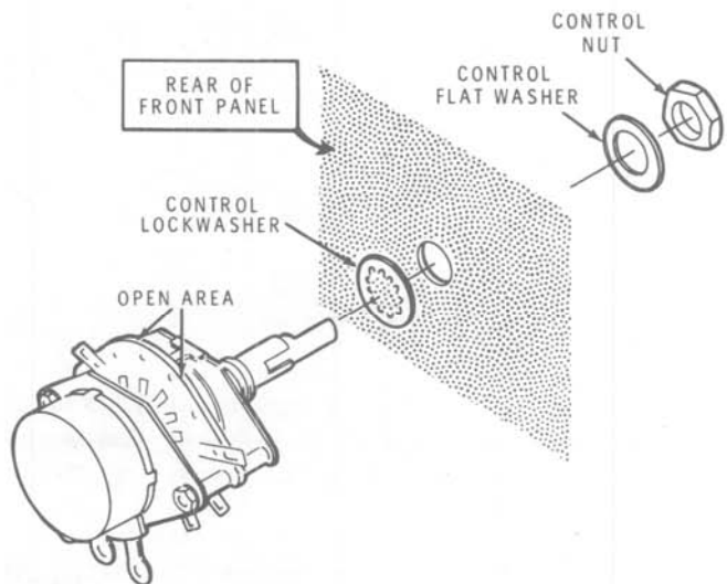
Detail 16C
