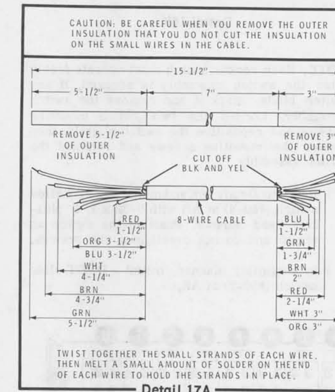
Detail 17A
