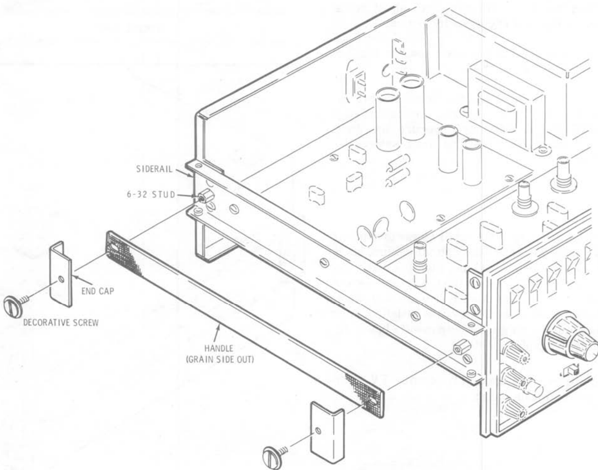
Detail 34A
