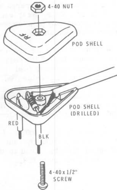
Detail 28C
