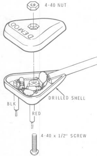
Detail 29B
