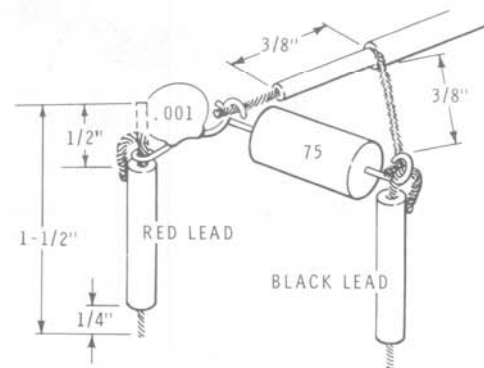
Detail 28B
