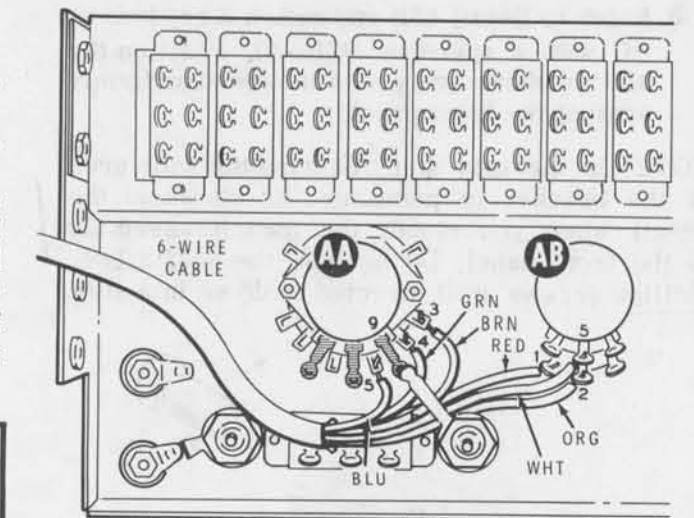
Detail 17B
