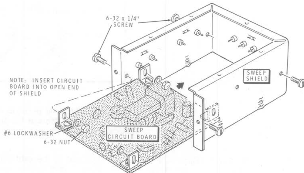
Detail 12D
