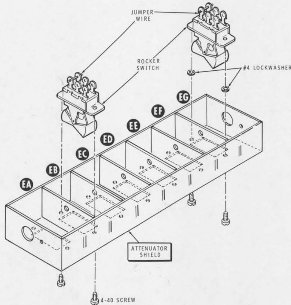
Detail 32D
