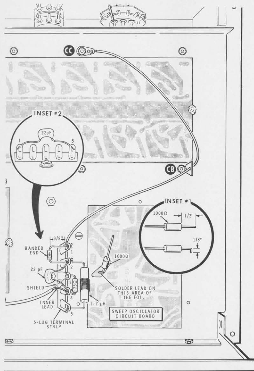
PICTORIAL 26
