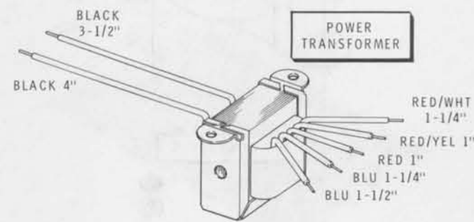
Detail 24A
