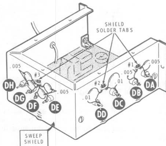
PICTORIAL 13
