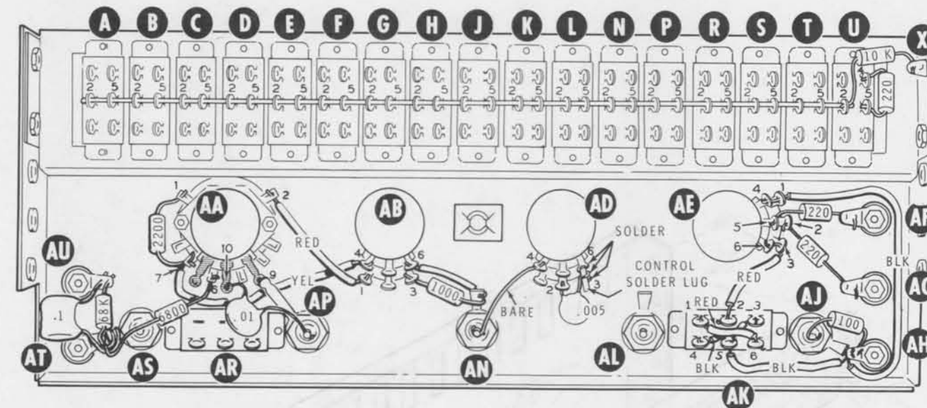
PICTORIAL 17
