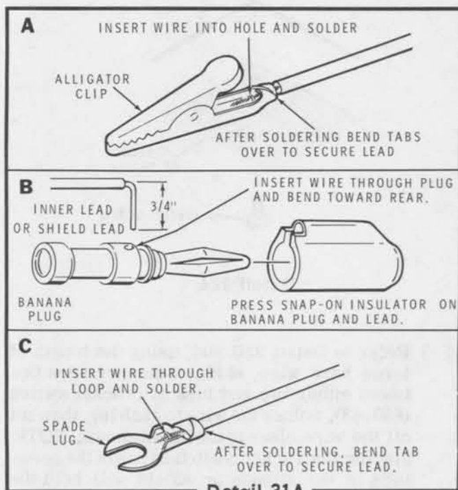
Detail 31A
