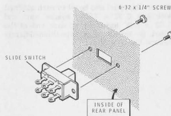
Detail 18D
