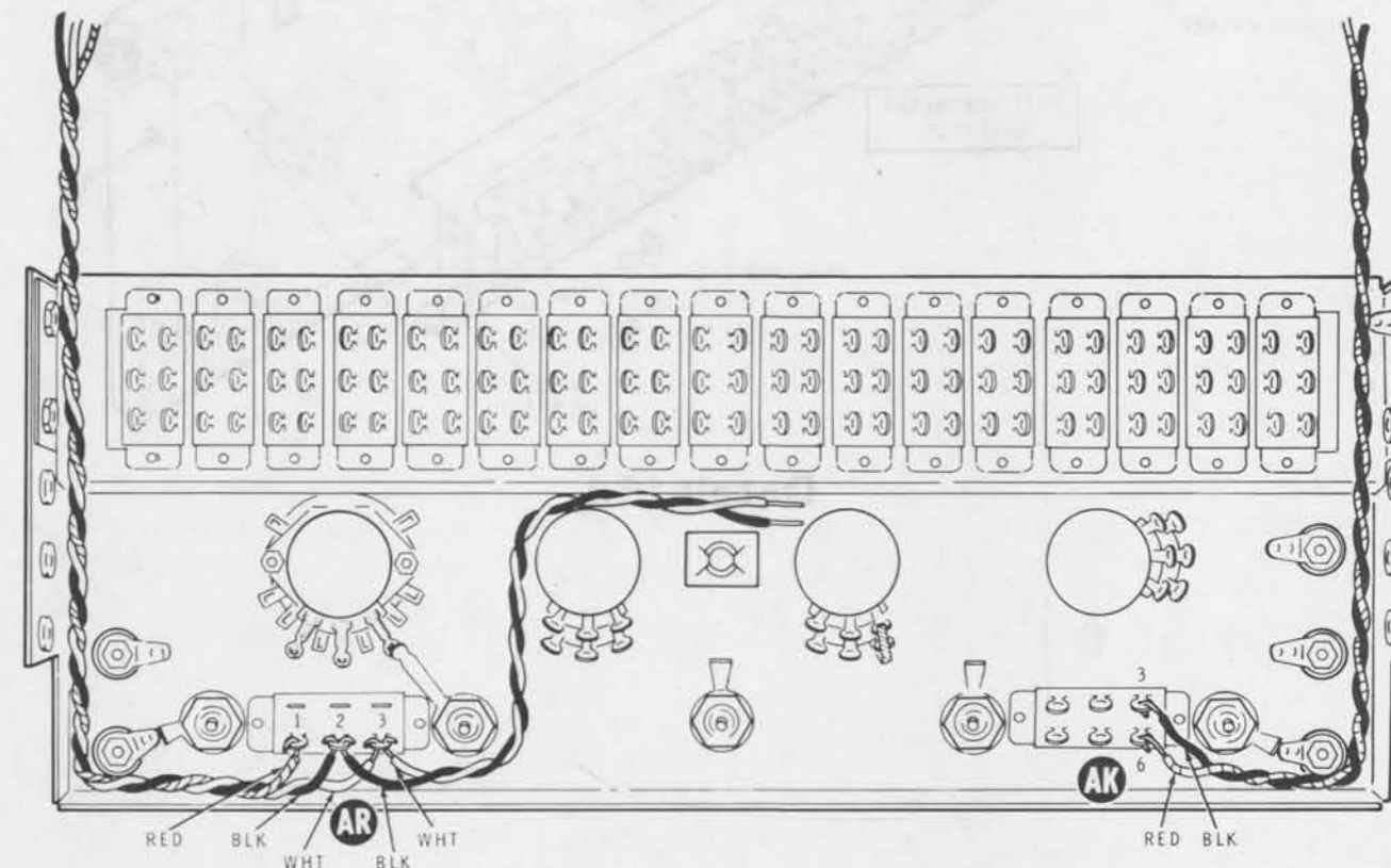
Detail 17D
