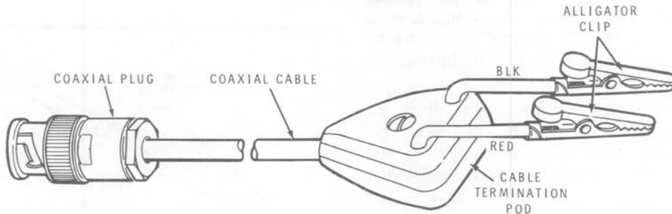
PICTORIAL 29
