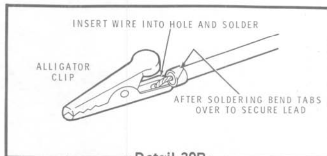
Detail 30B
