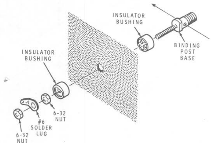
Detail 16A
