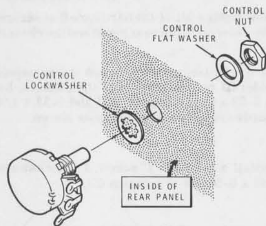
Detail 18C
