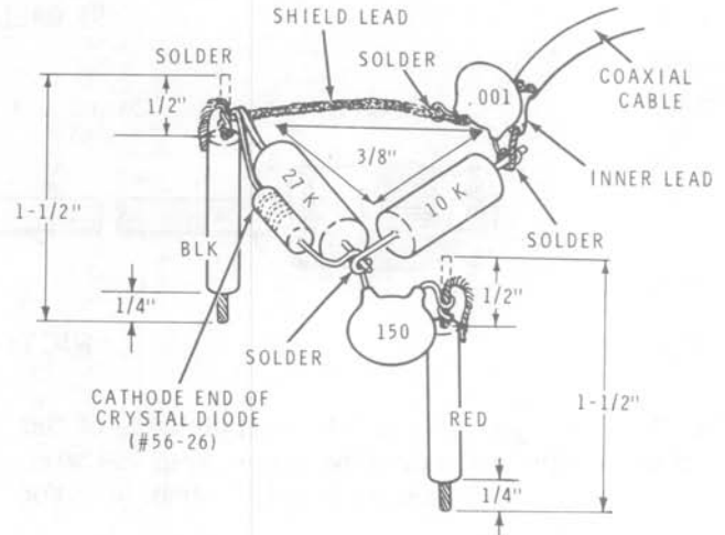
Detail 29A
