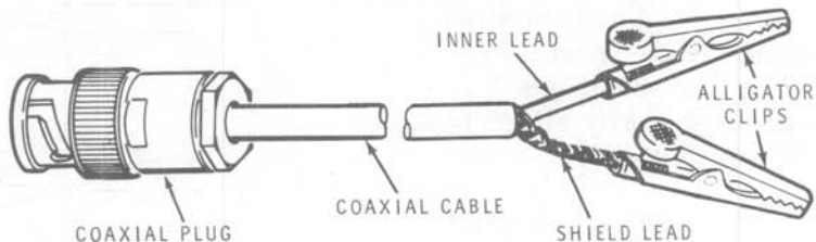
PICTORIAL 27
