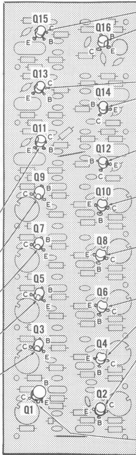
PICTORIAL 7
