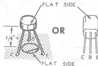
Detail 9B
