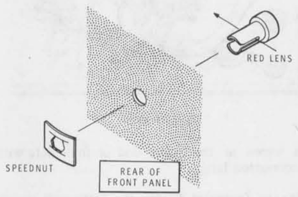
Detail 16H
