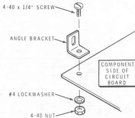
Detail 12A
