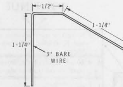
Detail 11A
