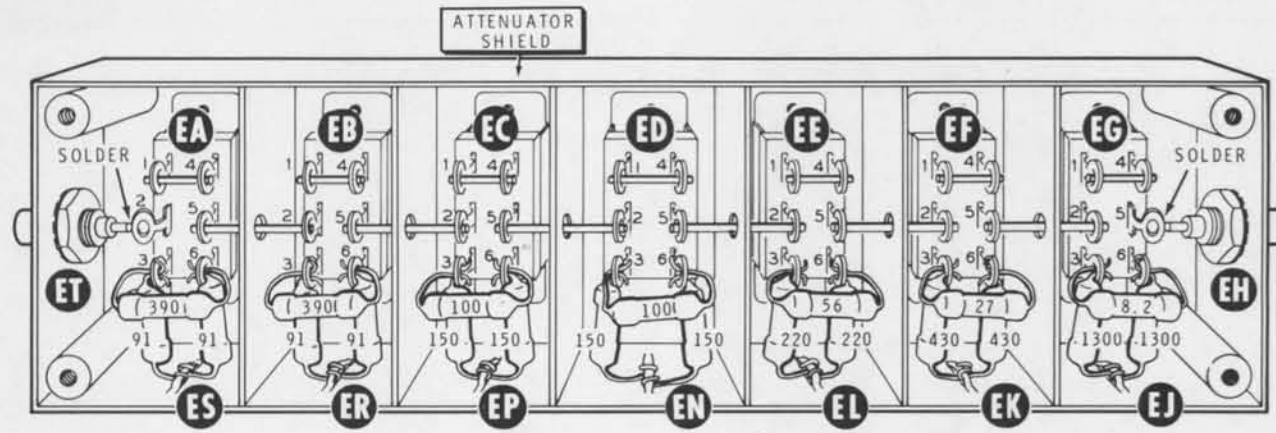
PICTORIAL 32
