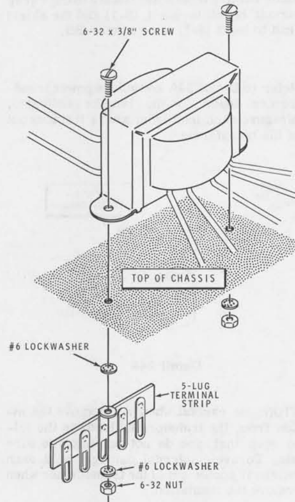
Detail 24B
