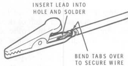
Detail 29C
