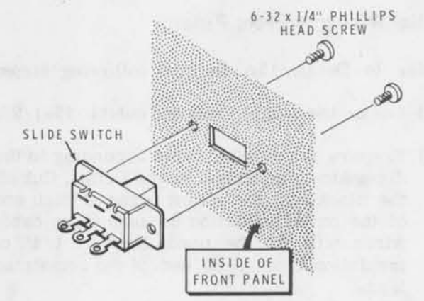
Detail 16K
