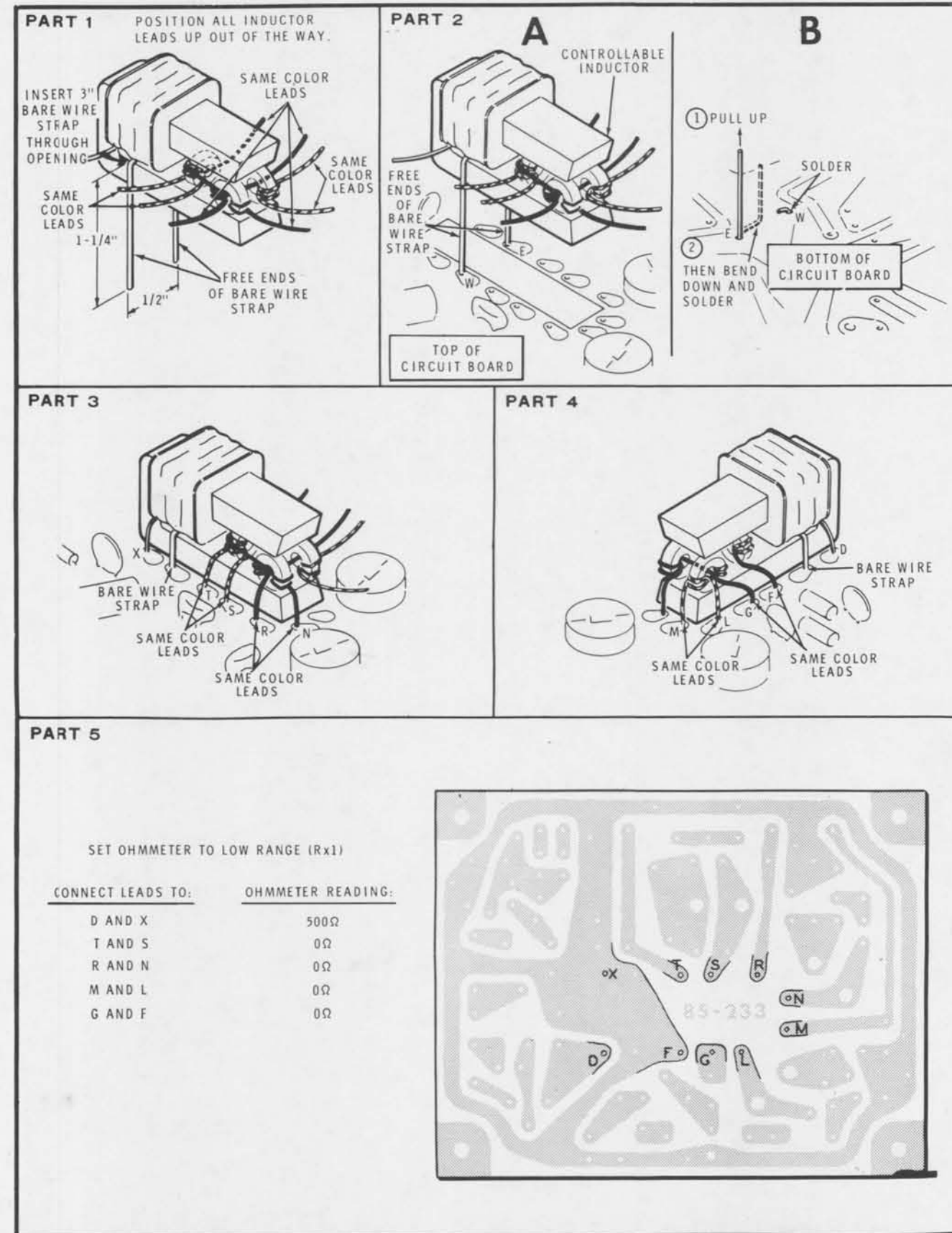
PICTORIAL 11
