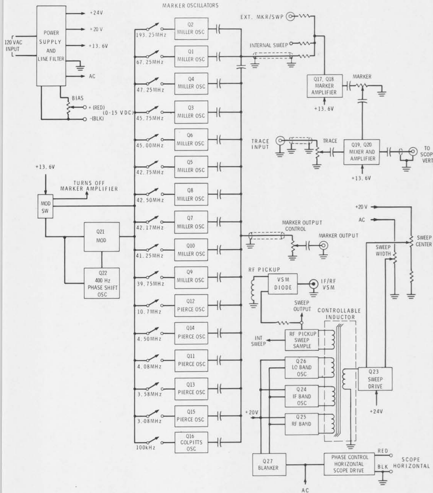
BLOCK DIAGRAM
