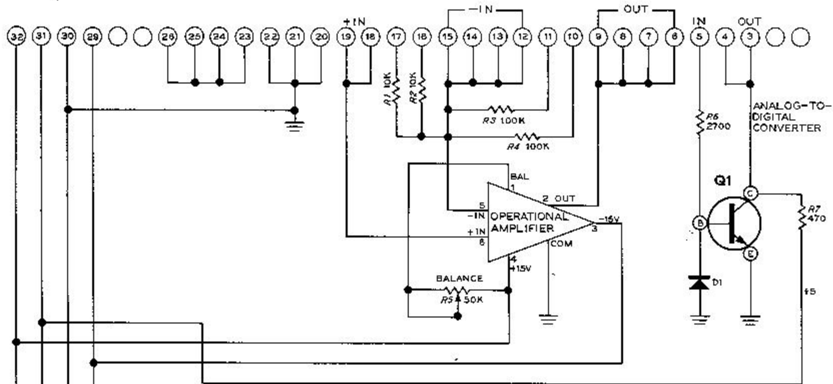
SCHEMATIC OF THE HEATH OPERATIONAL AMPLIFIER CARD MODEL EU-900-NA
