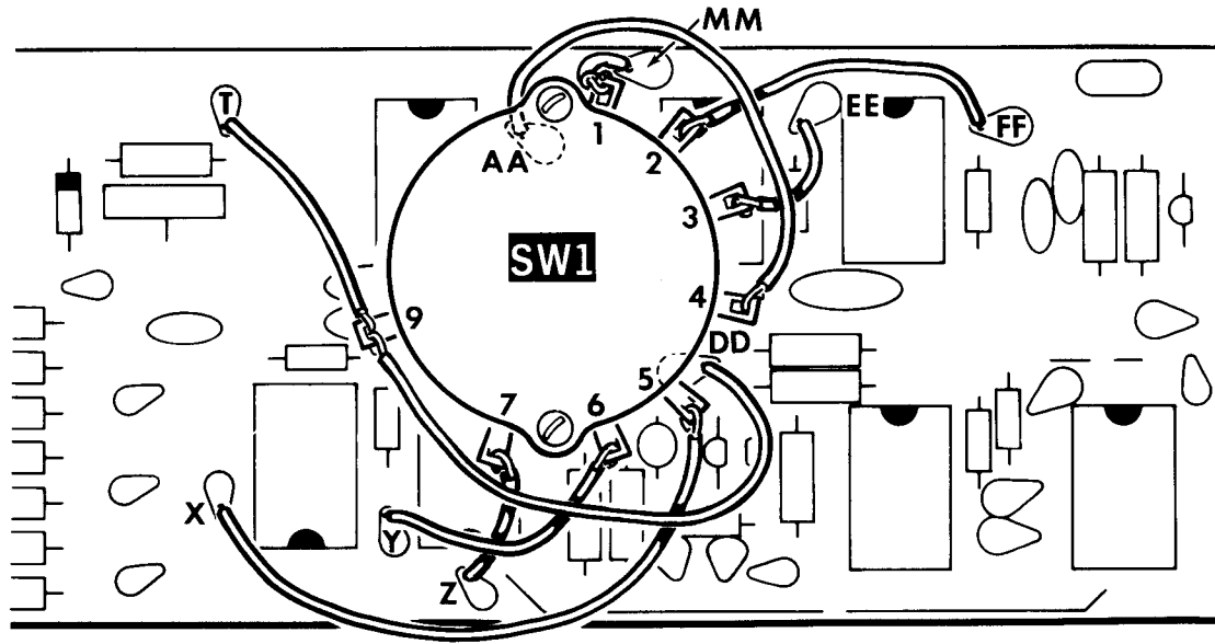
PICTORIAL 1-7
