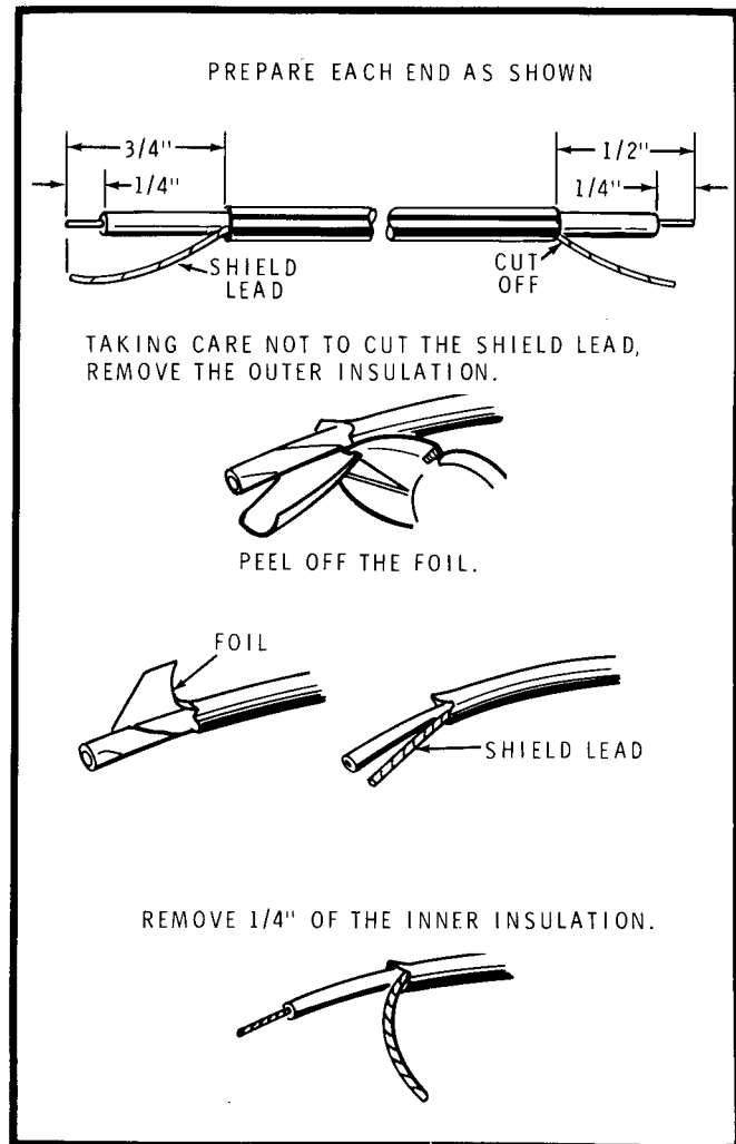
Detail 1-6A
