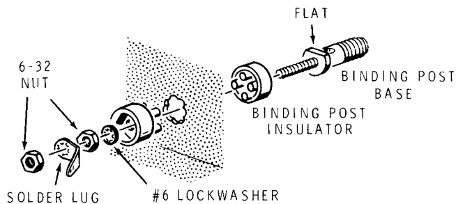
Detail 2-6D
