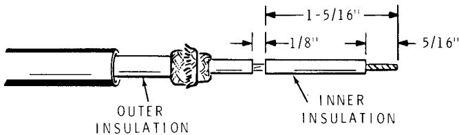
Detail 2-11B
