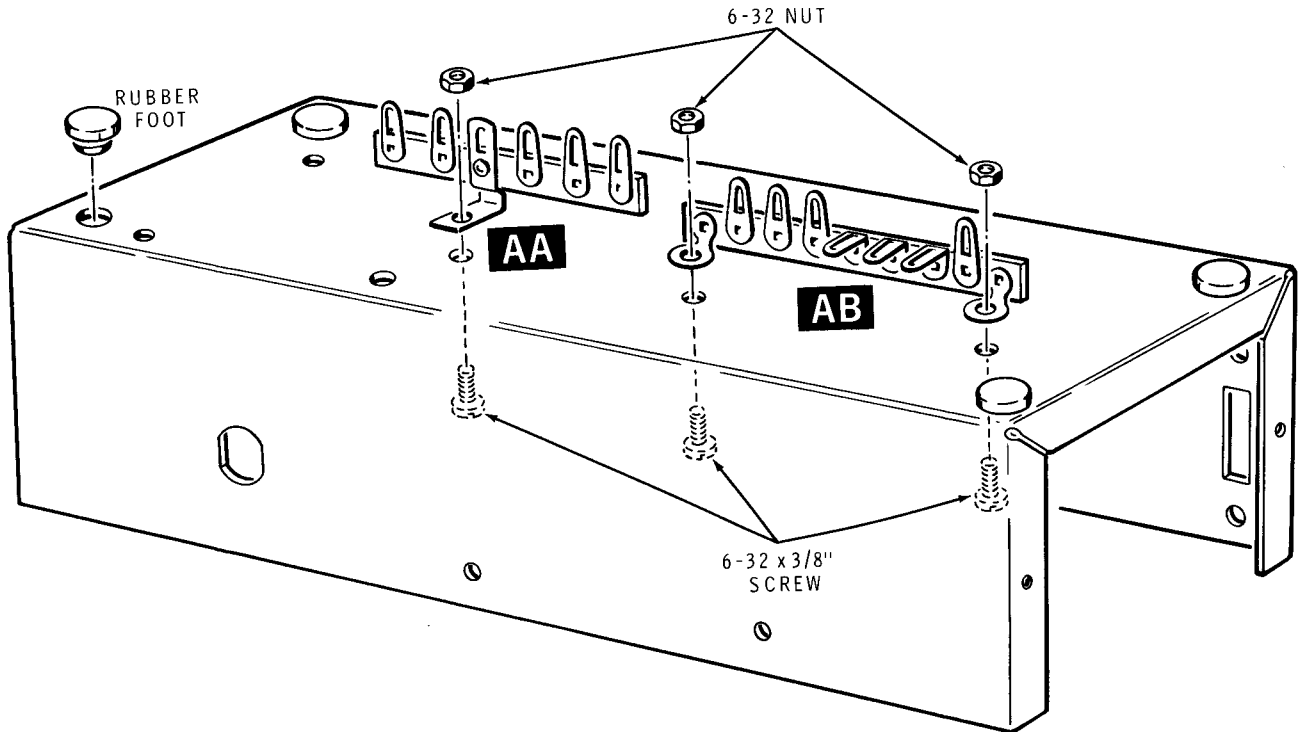
PICTORIAL 2-1
