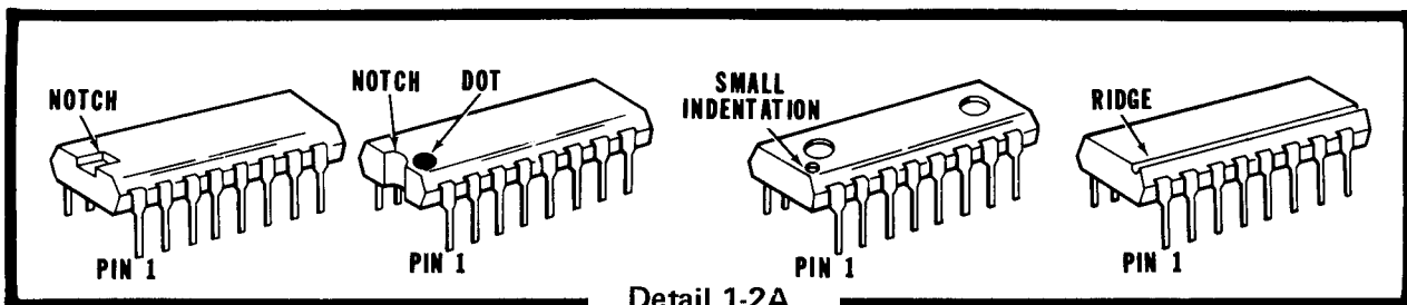
Detail 1-2A
