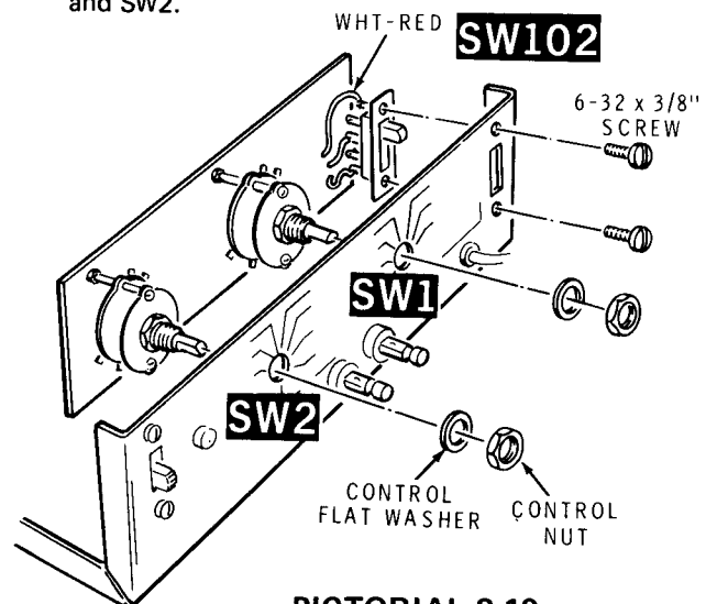
PICTORIAL 2-10
