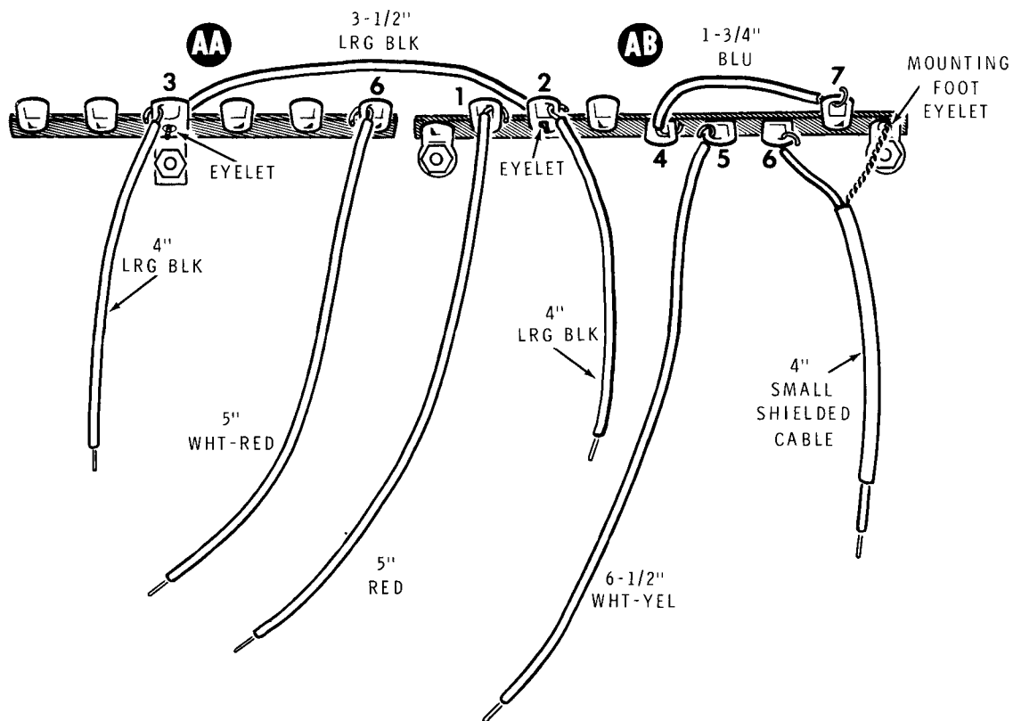
PICTORIAL 2-2
