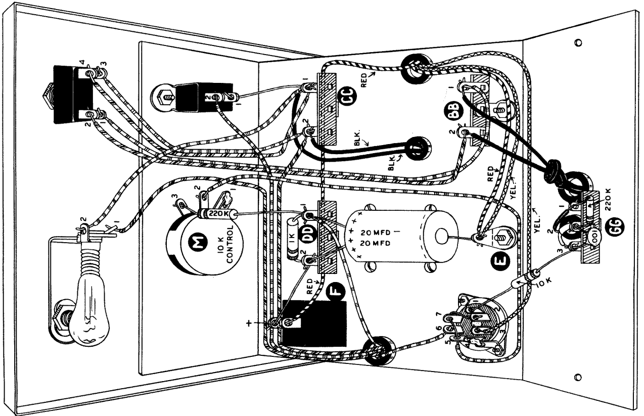
PICTORIAL 1
