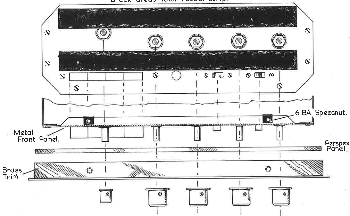
PICTORIAL-15.
