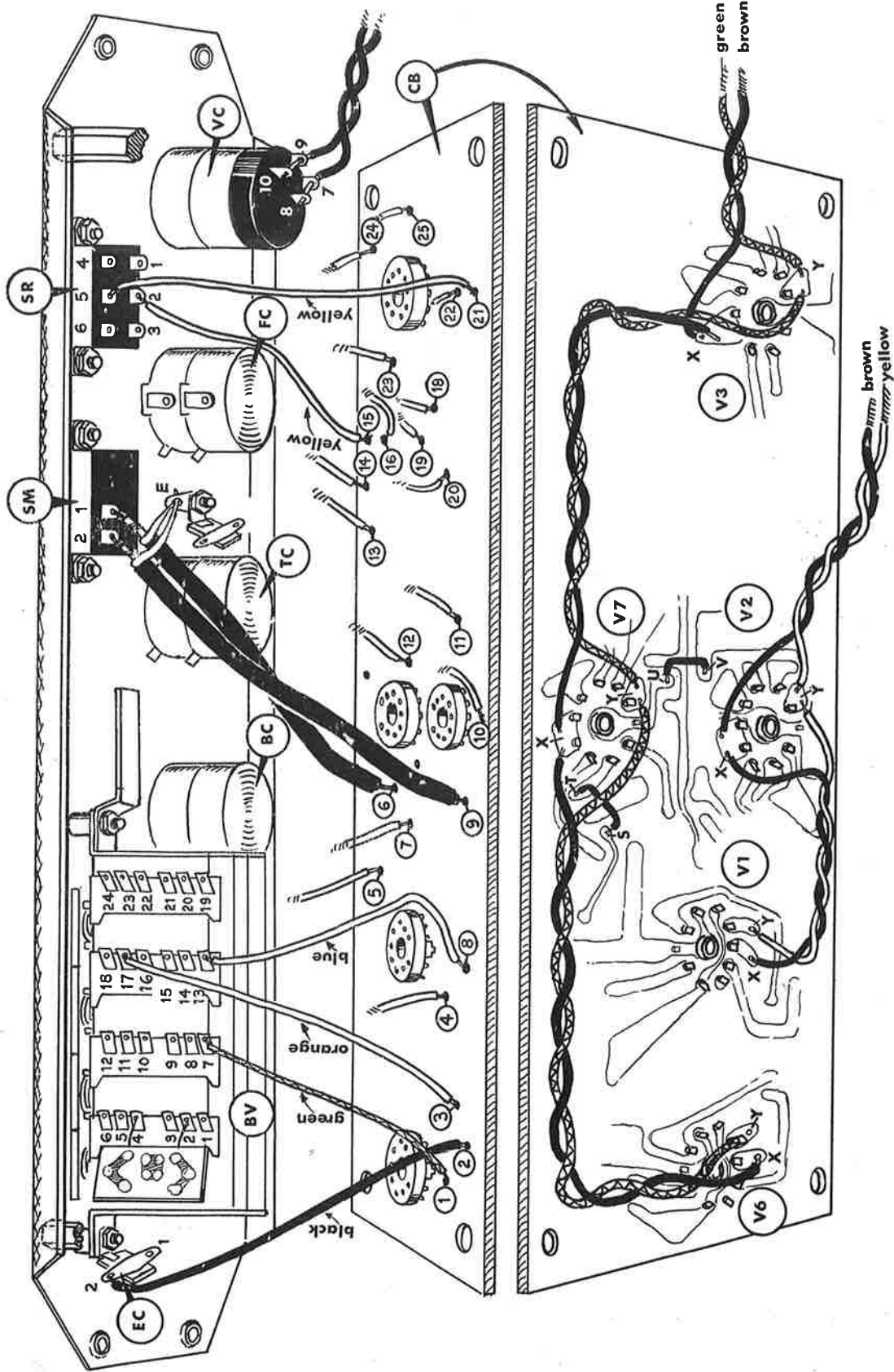
PICTORIAL-12.
