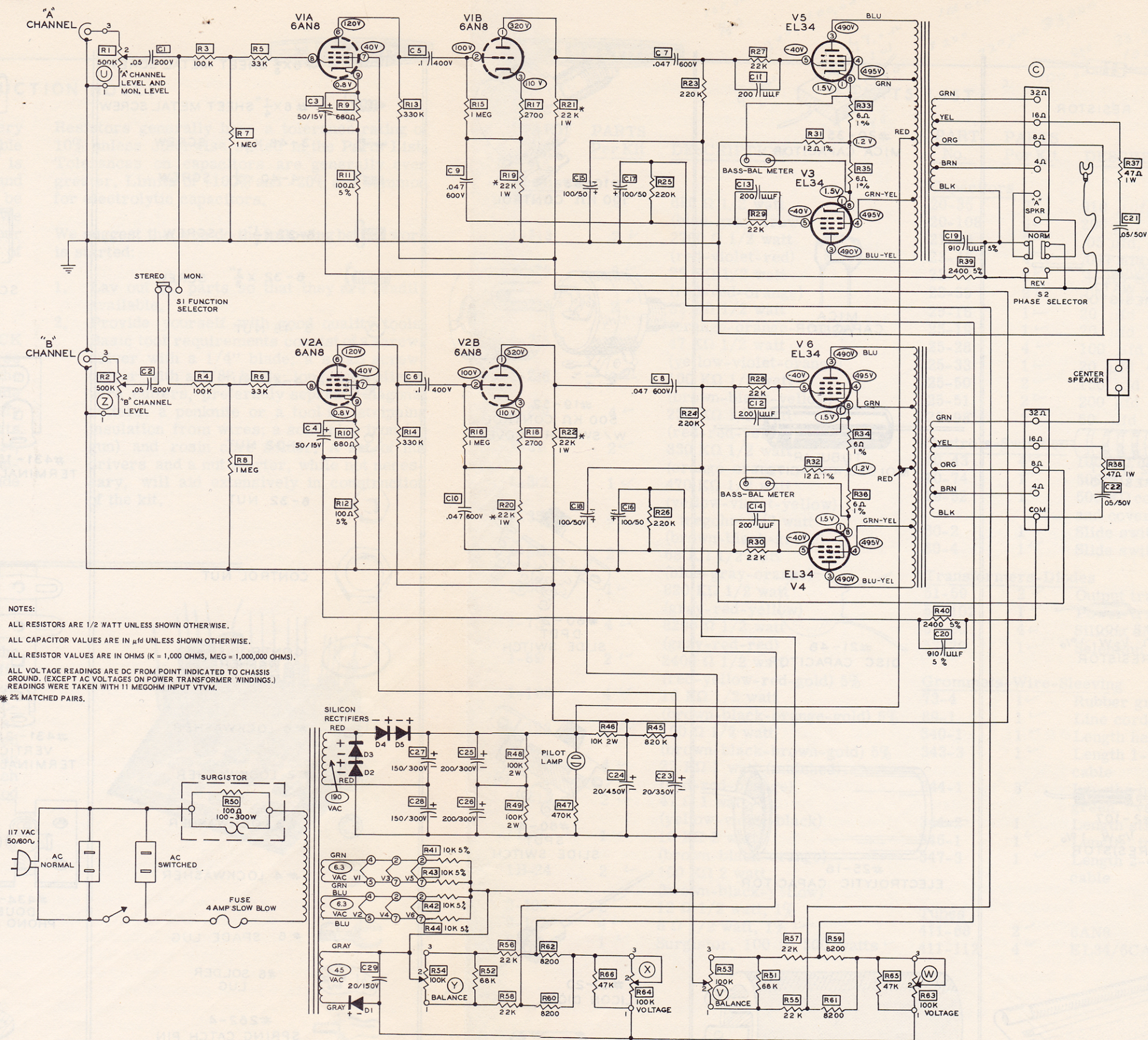
SCHEMATIC OF THE HEATHKIT® 80 WATT AMPLIFIER MODEL AA-121
