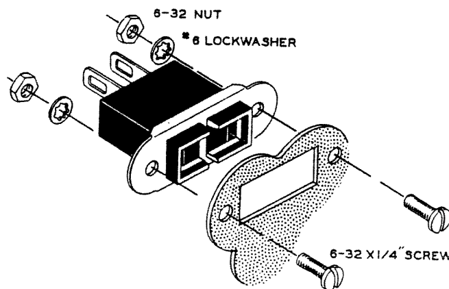
Detail 1C
