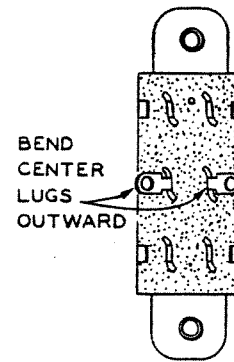
Detail 3A
