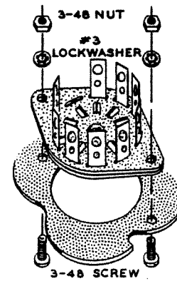
Detail 1F
