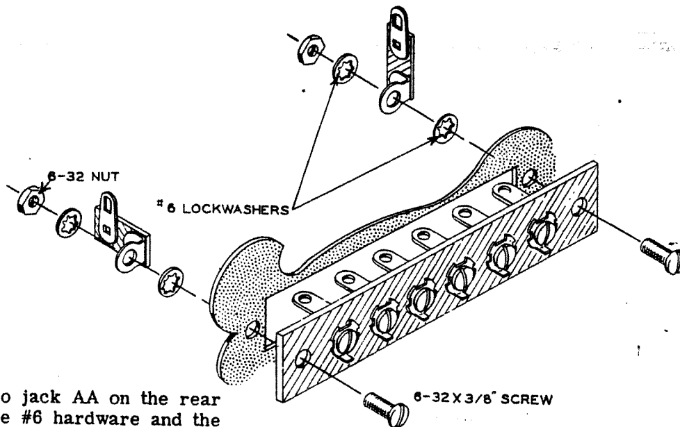
Detail 1B
