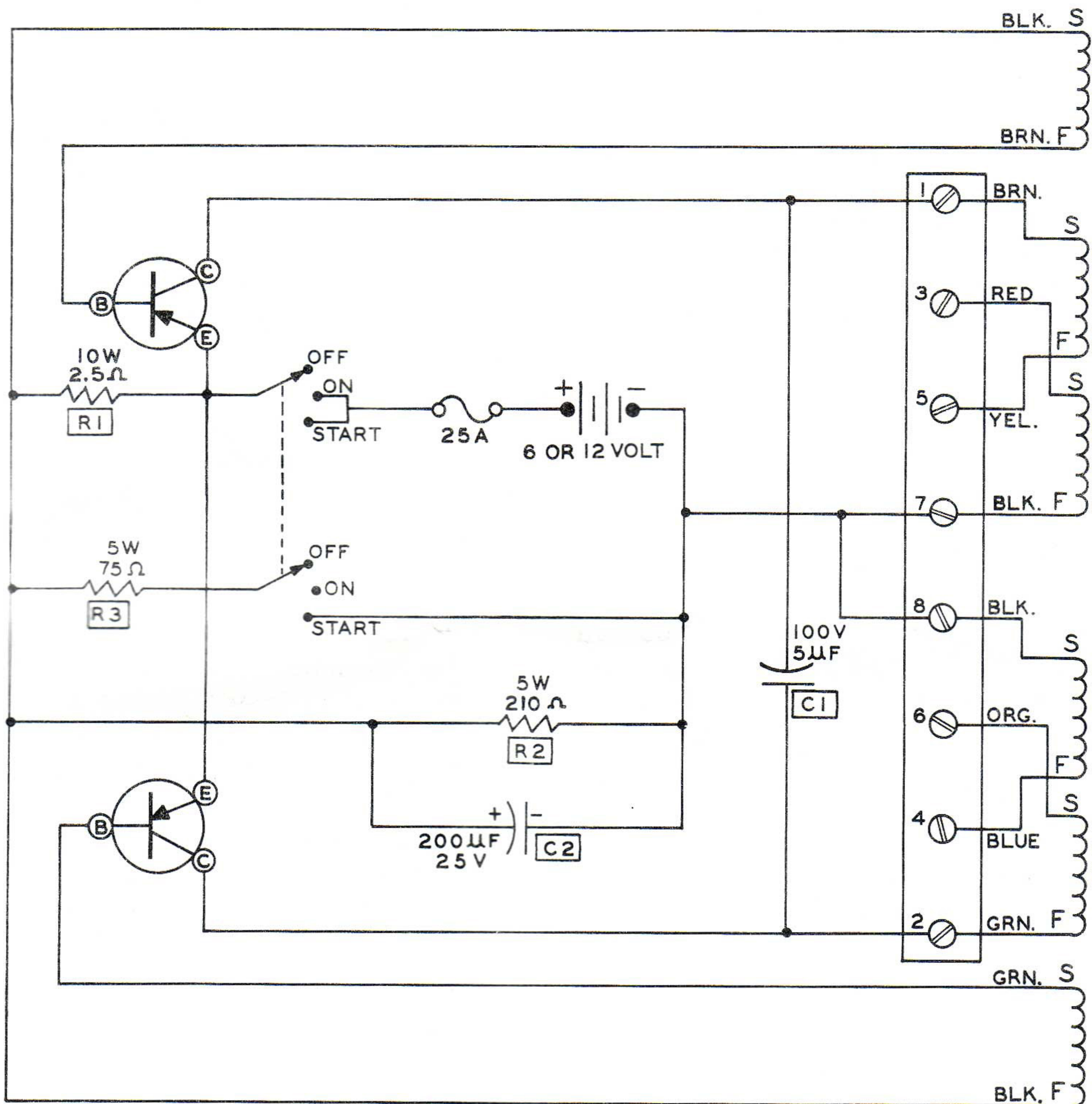
SCHEMATIC OF THE HEATHKIT® POWER INVERTER MODEL MP-10
