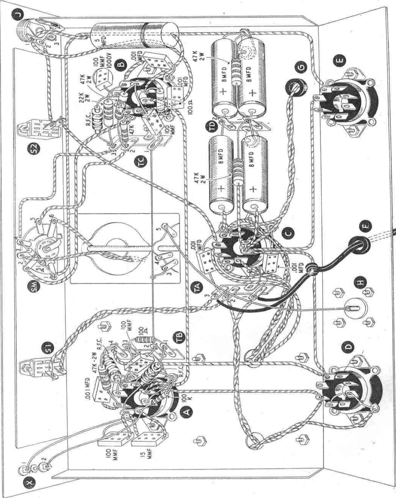
PICTORIAL 1
