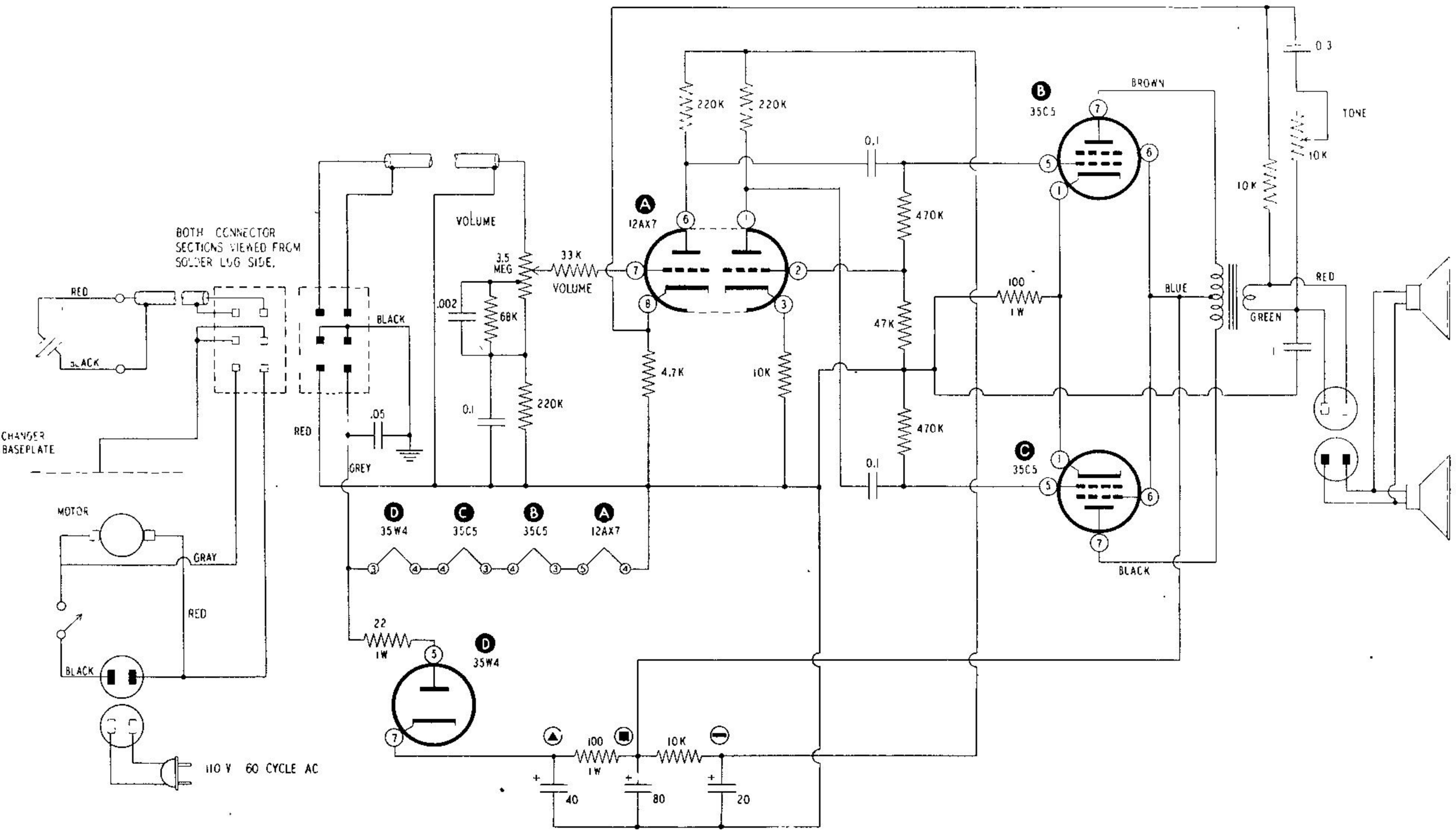
HEATHKIT RECORD PLAYER MODEL RP-1
