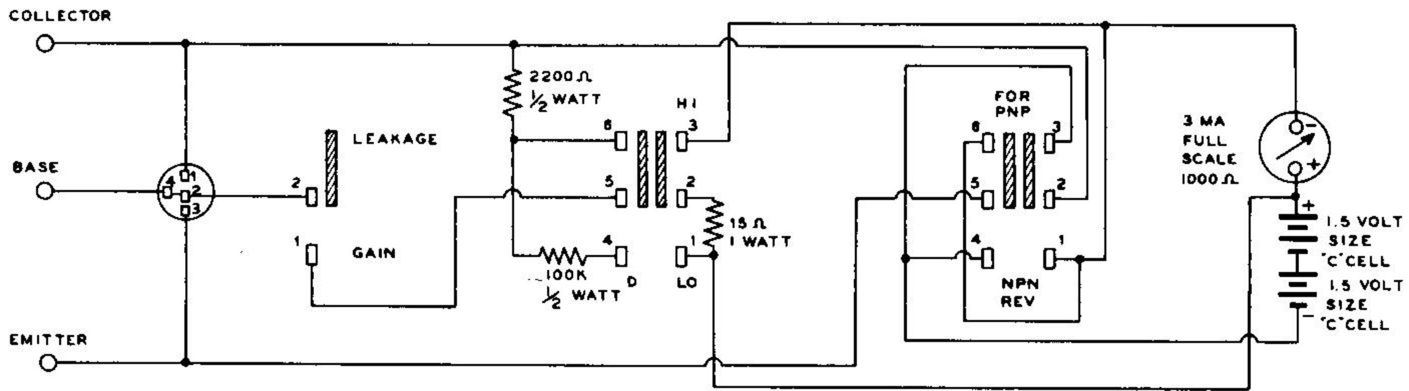
SCHEMATIC DIAGRAM
