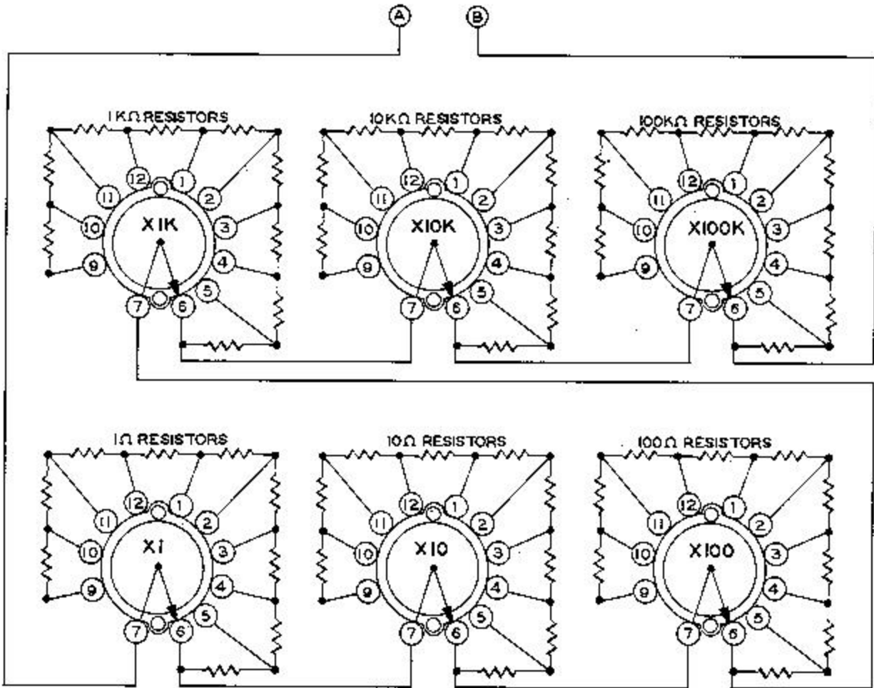
SCHEMATIC DIAGRAM MODEL IN-11
