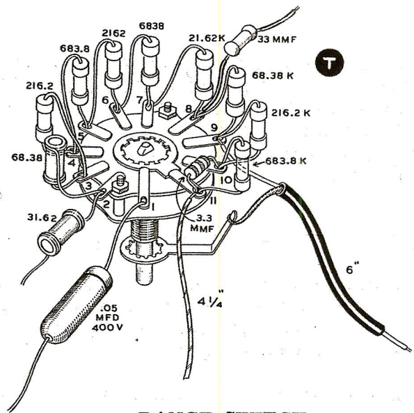
RANGE SWITCH
